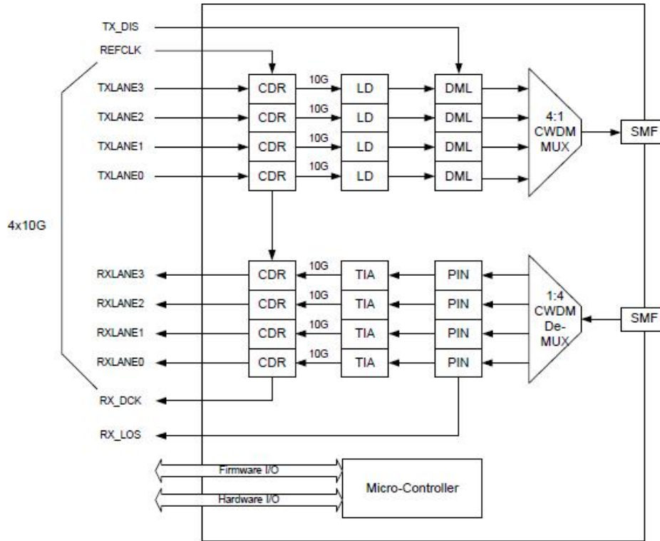
Transceiver functional diagram
