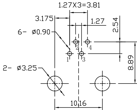
PC Board Layout (Top View)
