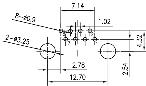
SUGGESTED PCB LAYOUT (TOP VIEW)
