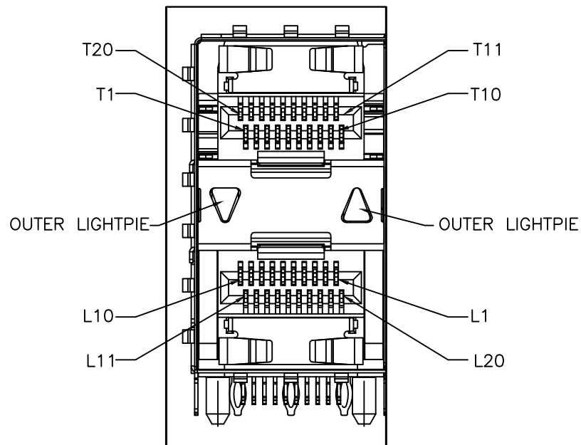
DETAIL A CIRCUIT NUMBERING AND LIGHTPIE INDENTIRCACTION
