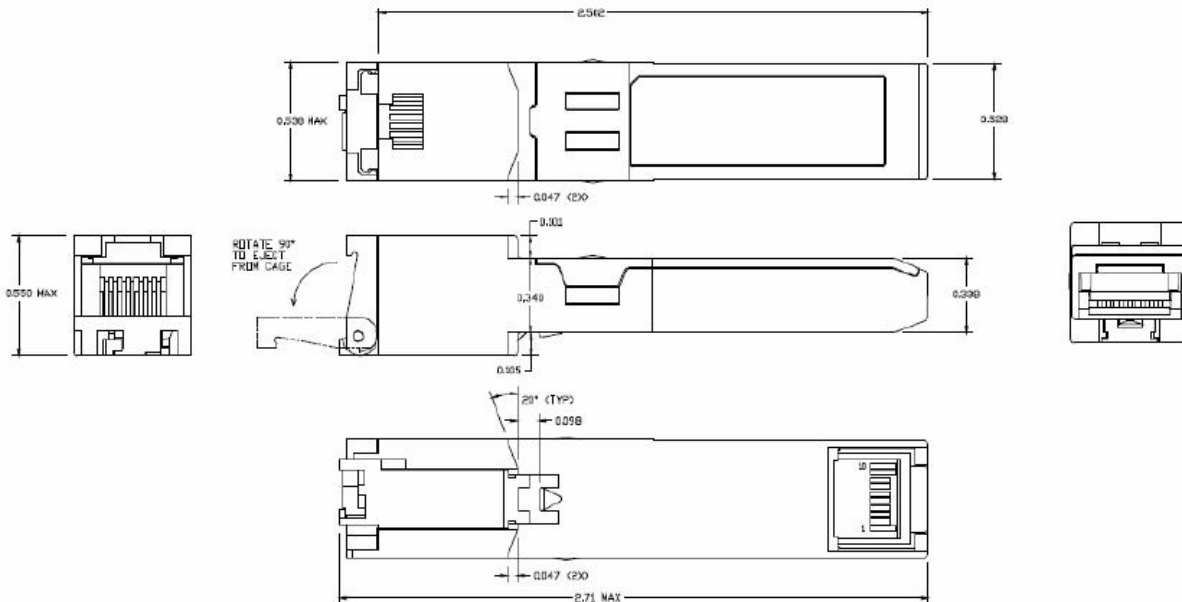
Figure 2. LP-RJ452G-TC mechanical dimensions
